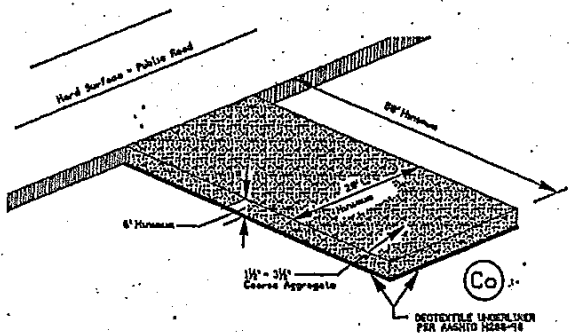
GRAVEL CONSTRUCTION ENTRANCE
